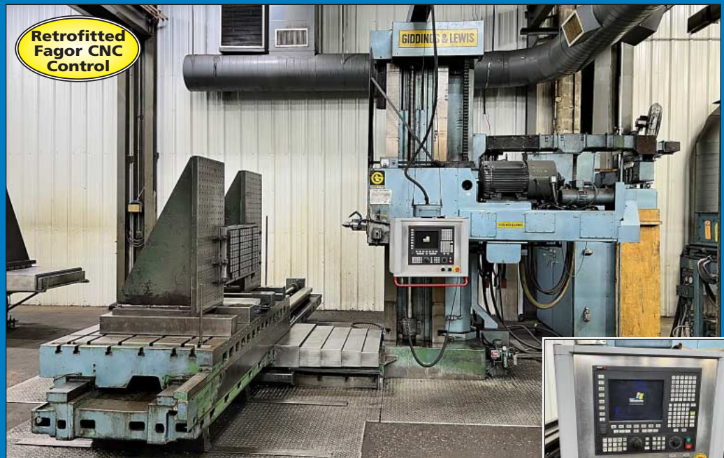
5" G&L Model PC-50 CNC Horizontal Boring Mill
